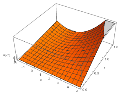
(c) Exact solution u(x, t) .
